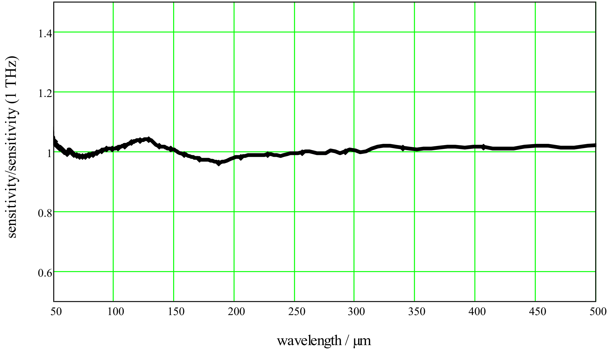
Normalized Sensitivity for a THz Absorber
